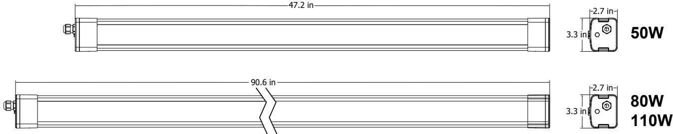
Figure 1 • Dimensions
