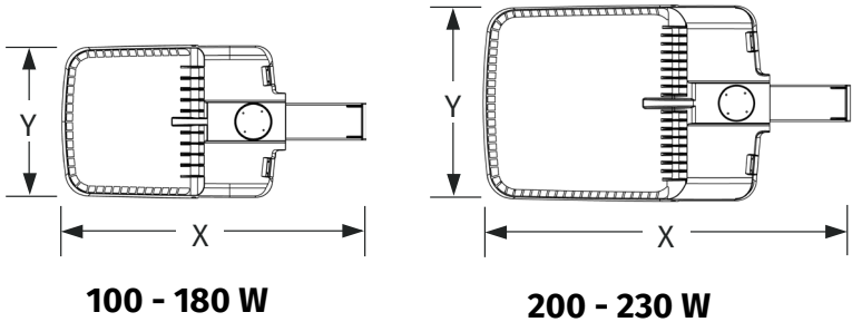
Figure 1 • Dimensions
