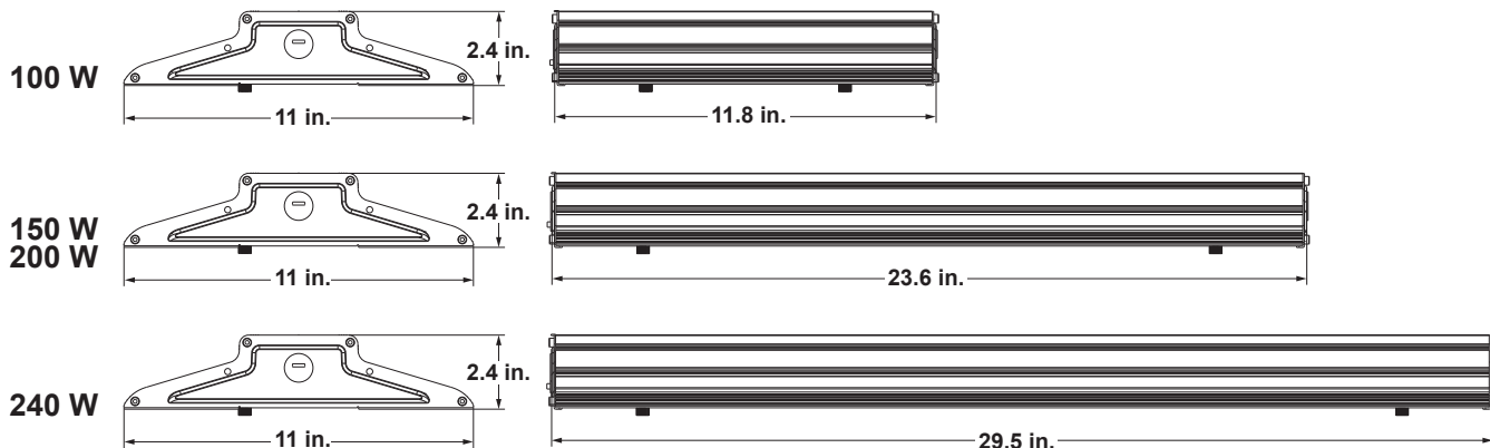
Figure 1 • Dimensions
