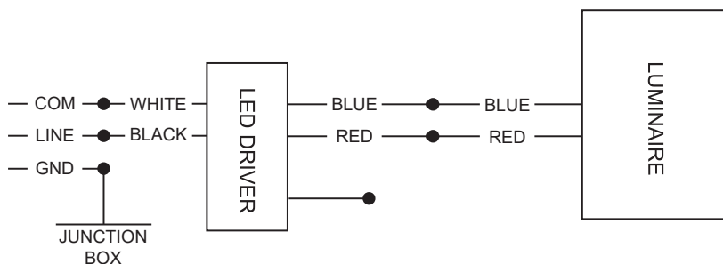
Figure 2 • Wiring Diagram
